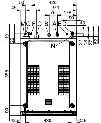
Connection positions in appliance floor
