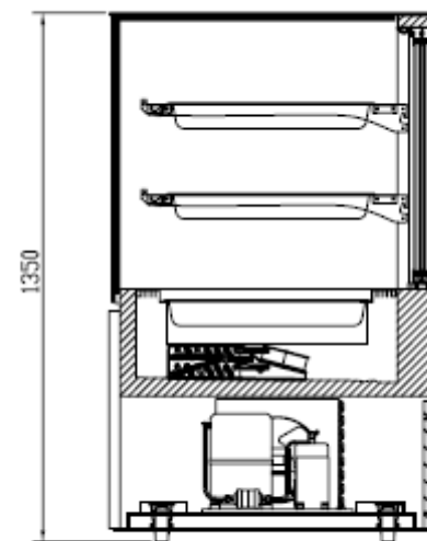
SECTION VIEW 左剖视图
