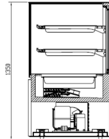
SECTION VIEW 左剖视图
