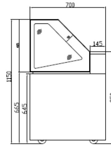
SIDE VIEW 左侧视图
