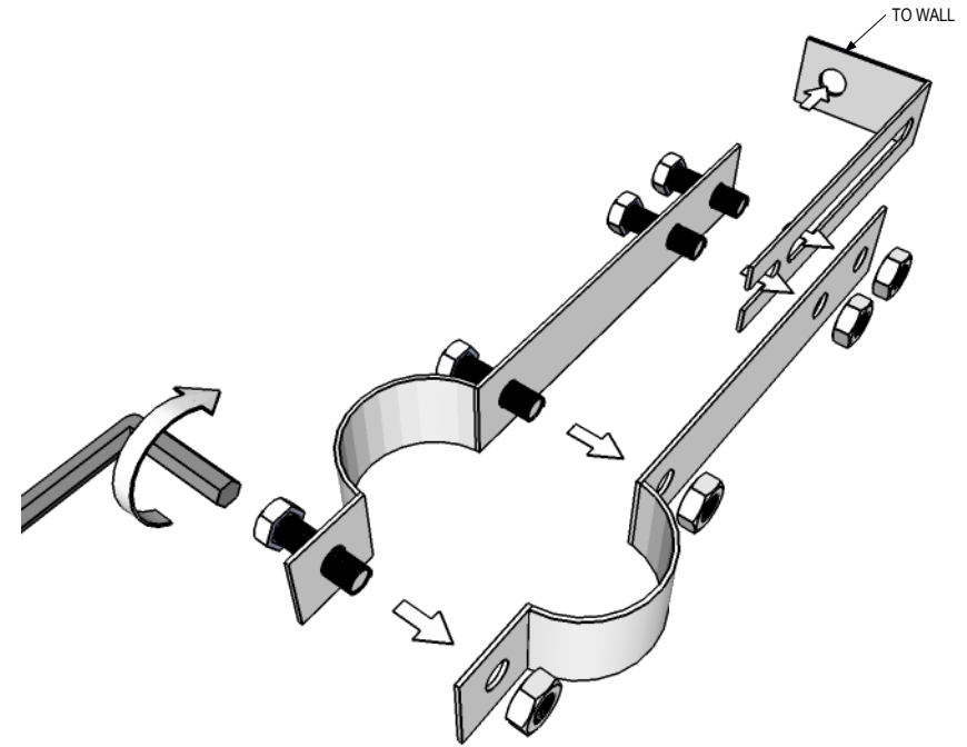
ASSEMBLING ISOMETRIC VIEW do not scale
