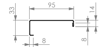
REINFORCING CHANNEL I DETAIL
