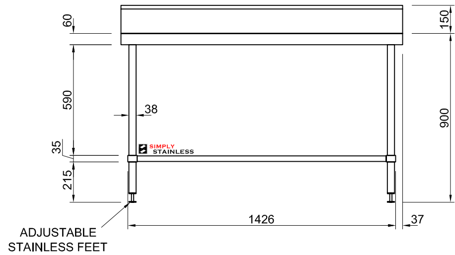
FRONT ELEVATION
