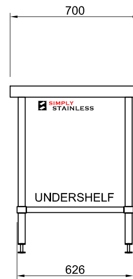
SIDE ELEVATION
