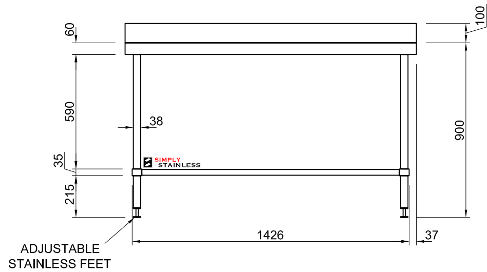
FRONT ELEVATION
